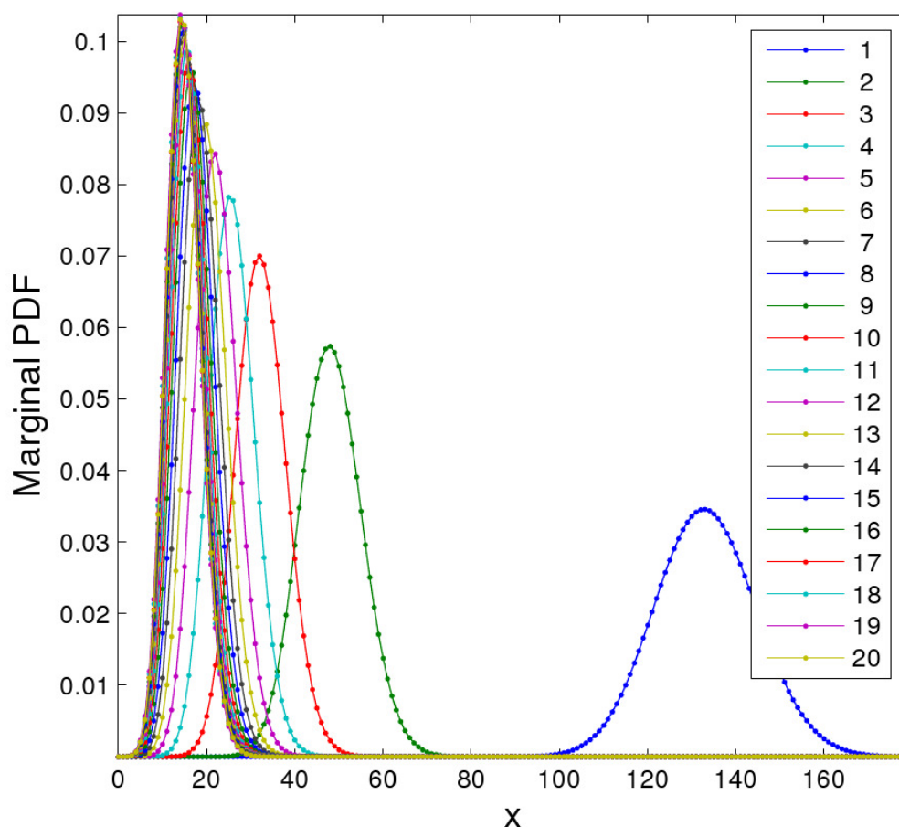
Figure 5. The simulation of a cascade composed by 20 terms shows the typical delay that has been observed for simpler examples.
