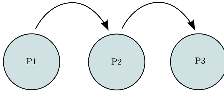
Figure 4. Schematic representation of a cascade.
