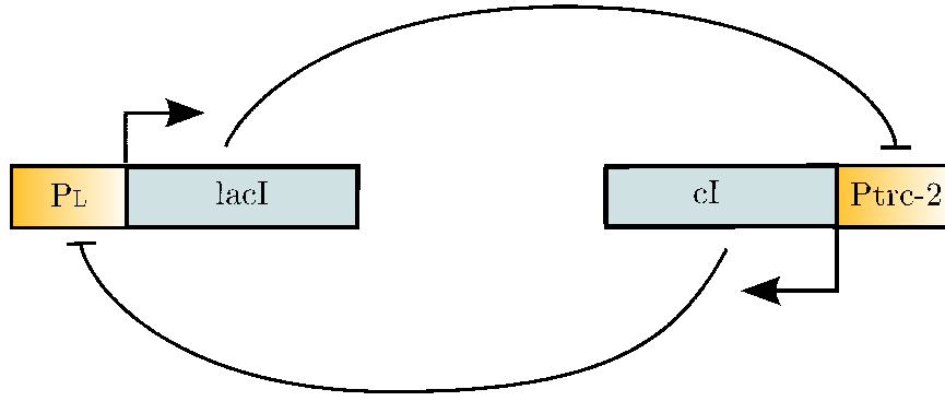
Figure 1. Schematic mechanism of the toggle switch [12]. The constitutive P_L promoter drives the expression of the lacI gene, which produces the lac repressor tetramer. The lac repressor tetramer binds the lac operator sites adjacent to the P_{trc-2} promoter, thereby blocking transcription of cI . The constitutive P_{trc-2} promoter drives the expression of the cI gene, which produces the \lambda -repressor dimer. The \lambda -repressor dimer cooperatively binds to the operator sites native to the P_L promoter, which prevents transcription of lacI .
