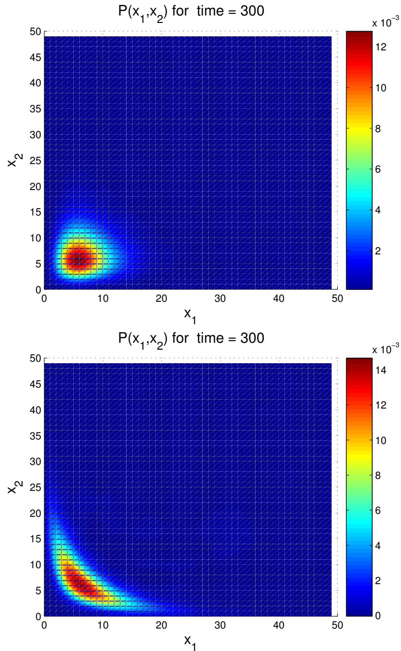
Figure 7. Final state of the toggle-switch model for a Hartree-like model (up) and the converged solution obtained by the proposed method (down). Axis represent the concentration of each competing protein.
