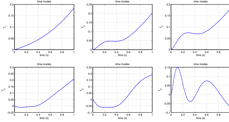
Fig. 2 Time modes: T_i^k(t) , i = 1, \dots, 6
