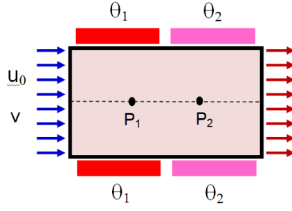
Fig. 11 Thermal process consisting of two heating devices located on the die walls where the temperature is enforced to the values \theta_1 and \theta_2 respectively.
