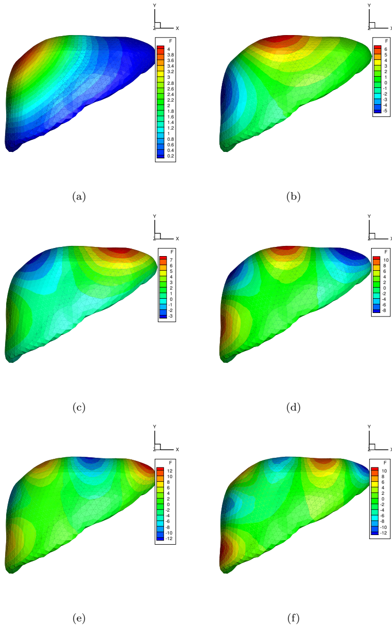
Fig. 15 Six first functions \mathbf{Y}(\mathbf{y}) , k = 1, \dots, 6 , for the simulation of the liver. Note that, in this case, functions \mathbf{Y}(\mathbf{y}) are defined on the boundary of the liver only.
