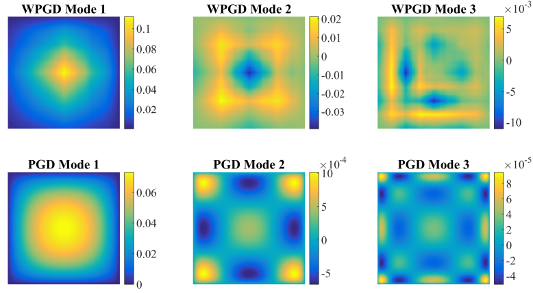
Figure 6. PGD modes X_i(x) \cdot Y_i(y) versus WPGD modes Z_i(x, y) .
