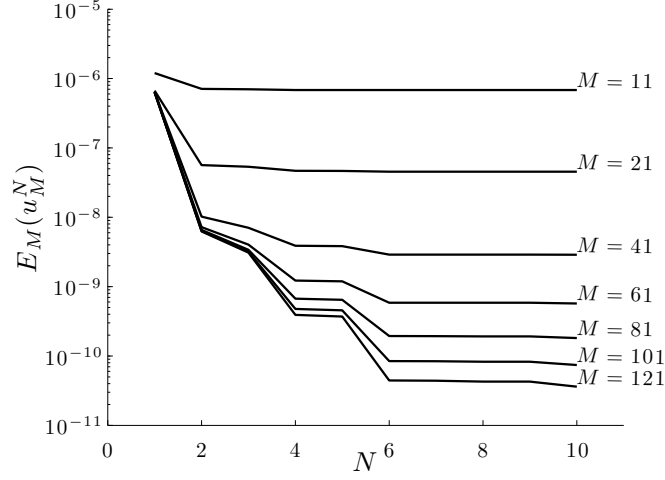
Figure 1. PGD error E_M(u_M^N) as a function of the number of enrichment steps N for different numbers M of discretization points.
