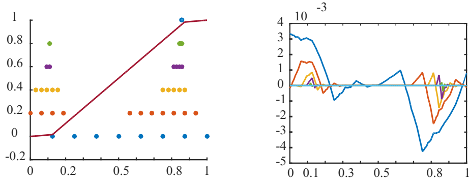
Figure 2. Adaptive approximation strategy.
