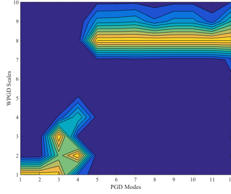
Figure 7. Contribution of different levels to each PGD mode.
