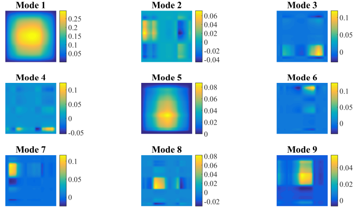
Figure 10. PGD modes: X_i(x) \cdot Y_i(y) .
