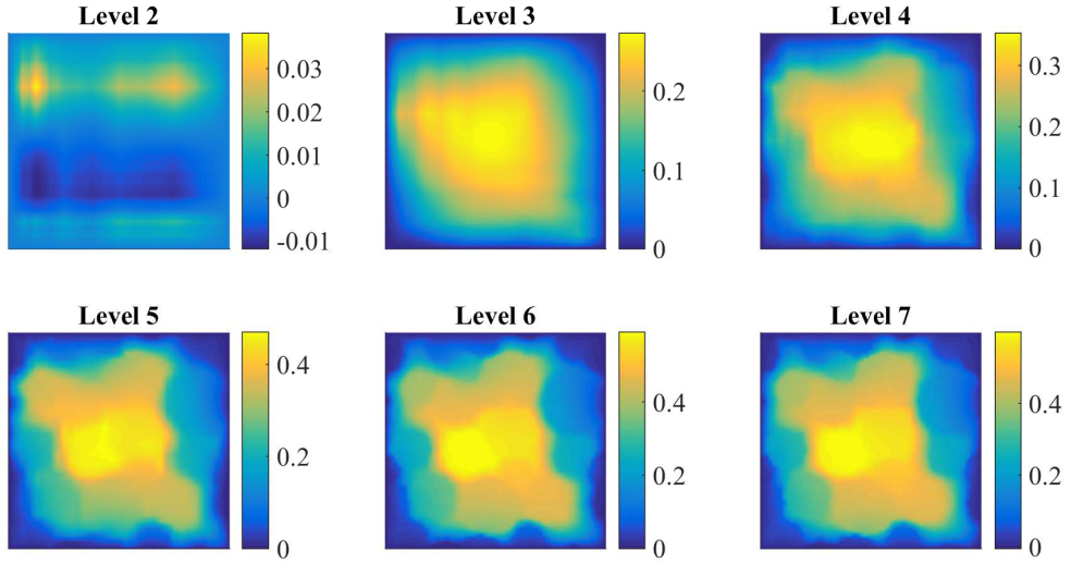
Figure 9. Reconstructed solution for different approximation levels.
