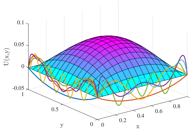
Figure 3. Reconstructed solution and involved modes in each direction.
