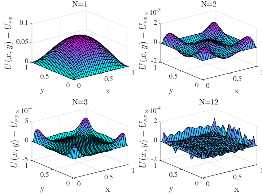
Figure 4. Difference between the reconstructed solution and the exact one for different number of models considered in the solution separated representation.
