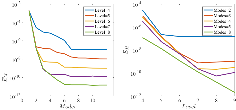
Figure 5. Convergence analysis with respect to the number of modes and levels.
