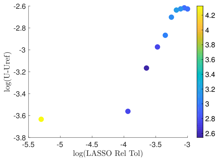
Fig. 5: Relative Tolerance of LASSO method versus solution error in logarithmic scale. The legend represent the time, in seconds, required to solve the LASSO minimization. 10 out of 75 time steps are sampled.
