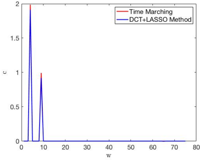
Fig. 8: DCT coefficients at a given spatial node equation with a good tolerance in LASSO. (Relative tolerance 0.8e-5 ).
