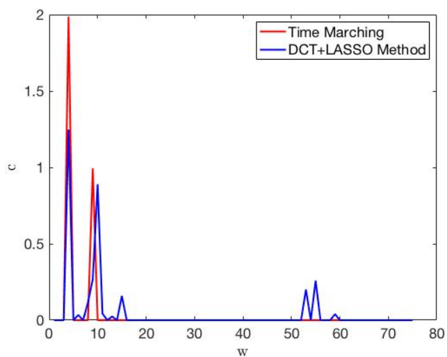
Fig. 7: DCT coefficients at a given spatial node with a bad tolerance in LASSO. (Relative tolerance 1e-4 ).
