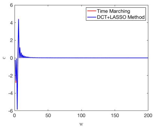
Fig. 18: c(\mathbf{x} = (0.5, 0.50), t) for transient Poisson's case. 150 time instants are sampled out of two hundred possible time steps.
