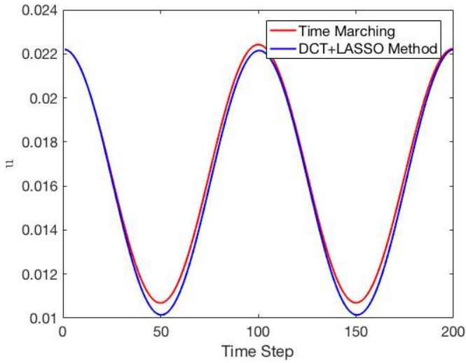
Fig. 13: u(\mathbf{x} = (0.5, 0.5), t) for the wave equation. 30 time instants are sampled out of two hundred possible time steps.
