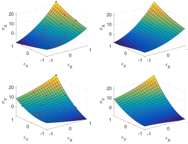
Fig. 3: Reference (left column) versus compressed sensing based reconstructed behavior manifold (right column). Red points indicate sampling locations.
