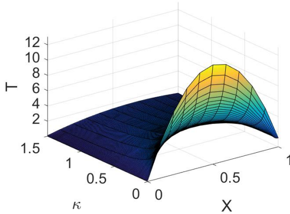
Fig. 1: Parametric solution u(x, \kappa) of Eq. (3).
