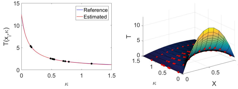
Fig. 2: Reference versus compressed sensing based reconstruction of the nodal solution evolution with the model parameter. Left: Solution at a given nodal position. Black nodes represent the sampling points. These are also indicated on the right.
