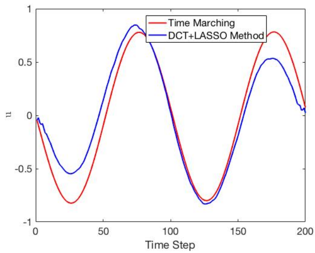
Fig. 15: u(\mathbf{x} = (0.5, 0.5), t) for transient Poisson's case. 100 time instants are sampled out of two hundred possible time steps.
